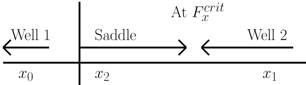
Figure 5.5: As F_x increases from 0 to F_x^{crit} , the saddle collides into the right well and disappears.
