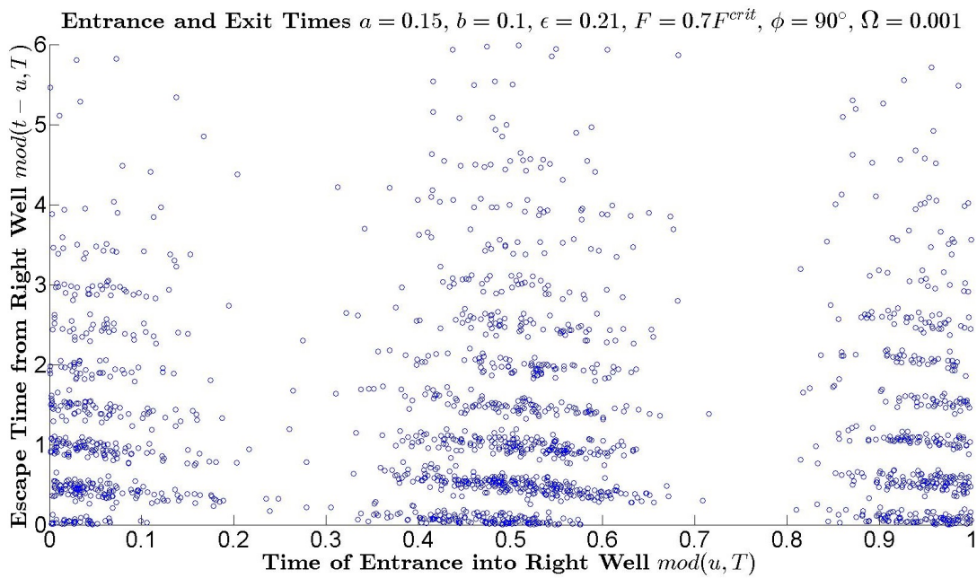
Figure 7.21: The u is the time of entrance into the well and t is the time of exit from the well.
