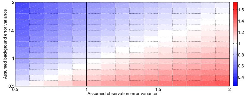
(a) Estimated observation error variance, \rho^e , as a function of assumed background and observation error variance. Red shows an overestimate, white an accurate estimate and blue an underestimate.
