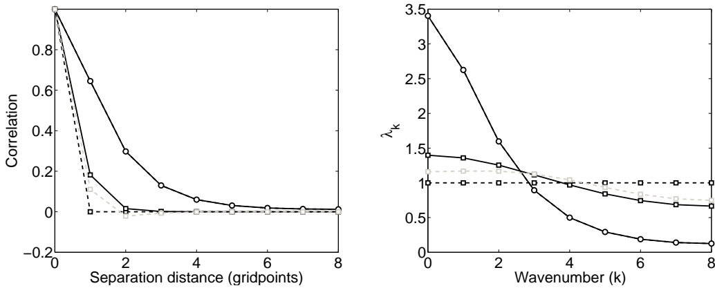
Figure 3: Correlation functions (left) and corresponding eigenvalues (right) for the Control Experiment. Estimated observation error (gray dashed line squares), when \tilde{\mathbf{B}} = \mathbf{B} (solid line circles), with L = 2 for \mathbf{R} (solid line squares) and \tilde{\mathbf{R}} = I (black dashed line squares).
