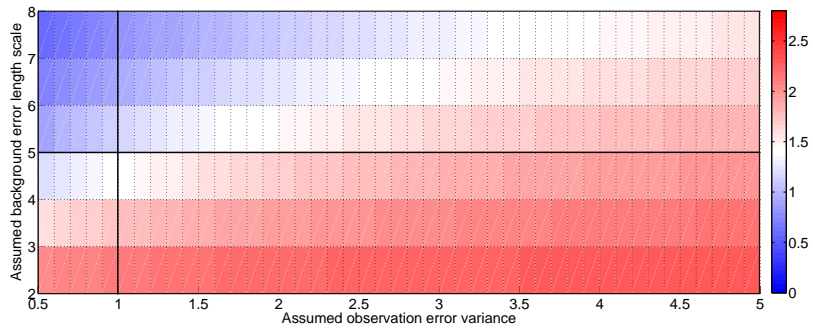
(b) First eigenvalue, \gamma_0^e , of the estimated observation error correlation matrix as a function of assumed observation error variance and background correlation length scale. Red shows an overestimate, white an accurate estimate and blue an underestimate.
