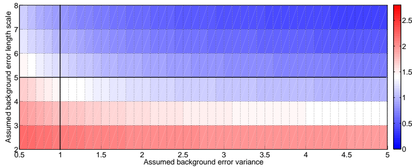
(b) First eigenvalue, \gamma_0^e , of the estimated observation error correlation as a function of assumed background error variance and correlation length scale. Red shows an overestimate, white an accurate estimate and blue an underestimate.
