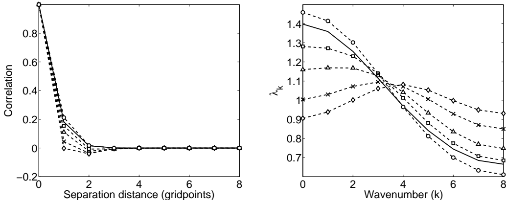
Figure 7: Estimated observation error correlations and corresponding eigenvalues for Experiments \beta 0.5 ( \tilde{\beta} = 0.5 , dashed line circles), \beta 0.75 ( \tilde{\beta} = 0.75 , dashed line squares), Control ( \tilde{\beta} = 1.0 , dashed line triangles), \beta 1.5 ( \tilde{\beta} = 1.5 , dashed line crosses) and \beta 2 ( \tilde{\beta} = 2.0 , dashed line diamonds) when the variance in the background error covariance matrix is misspecified in the assimilation. The exact observation correlation function \mathbf{C}_r (solid line) is plotted for comparison.
