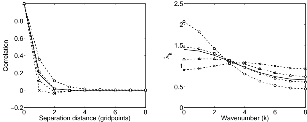
Figure 5: Estimated observation error correlations and corresponding eigenvalues for Experiments \rho0.5 ( \tilde{\rho} = 0.5 , dashed line crosses), Control ( \tilde{\rho} = 1 , dashed line triangles), \rho2 ( \tilde{\rho} = 2 , dashed line squares) and \rho10 ( \tilde{\rho} = 10 , dashed line circles) when observation errors are assumed uncorrelated and the variance misspecified in the assimilation. The exact observation error correlation function \mathbf{C}_r (solid line) is plotted for comparison.
