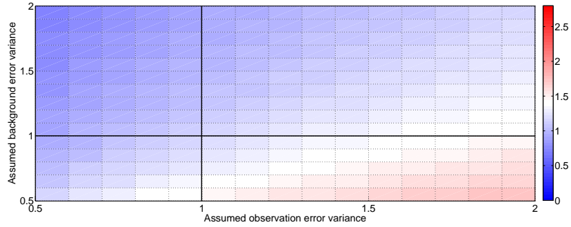
(b) First eigenvalue, \gamma_0^e , of the estimated observation error correlation as a function of assumed background and observation error variance. Red shows an overestimate, white an accurate estimate and blue an underestimate.
