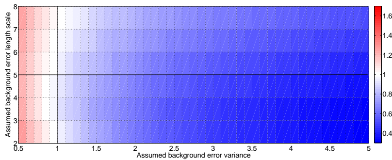
(a) Estimated observation error variance, \rho^e , as a function of assumed background error variance and correlation length scale. Red shows an overestimate, white an accurate estimate and blue an underestimate.
