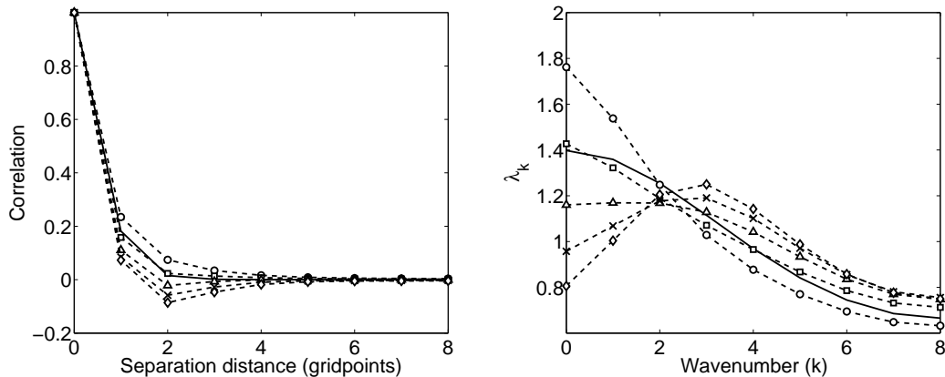
Figure 8: Estimated observation error correlations and corresponding eigenvalues for Experiments L3 (assumed background correlation length scale L = 3 , dashed line circles), L4 ( L = 4 , dashed line squares), Control ( L = 5 , dashed line triangles), L6 ( L = 6 , dashed line crosses) and L7 ( L = 7 , dashed line diamonds) when the length scale in the background error covariance matrix is misspecified in the assimilation. The exact observation error correlation function C_r (solid line) is plotted for comparison.
