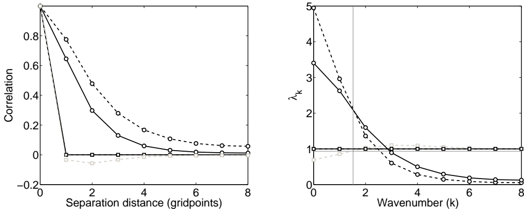
Figure 2: Correlation functions (left) and eigenvalues of the corresponding covariance matrices (right). Estimated observation error correlations (gray dashed line squares) when \mathbf{R} = \tilde{\mathbf{R}} = I (solid line squares) and the length scale in the assumed background error covariance (black dashed line circles) is L = 7 compared to the actual background covariance function (solid line circles) where L = 5 . On the right panel the thin horizontal line shows the \frac{1}{\rho^e} = 0.93 value and the vertical line divides the plot into regions where \lambda_k^e < \frac{1}{\rho^e} (left of line) and \lambda_k^e > \frac{1}{\rho^e} (right of line).
