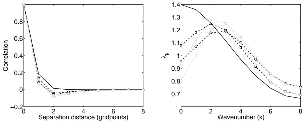
Figure 13: Rows of the exact (solid) and estimated observation error covariance matrices (left panel) for Experiments \rho2\beta1.5L6 (dashed black line squares), \rho2\beta2L6 (dashed black line circles), \rho2\beta1.5L7 (dash gray line squares) and \rho2\beta2L7 (dash gray line circles). The corresponding eigenvalues are also plotted (right panel).
