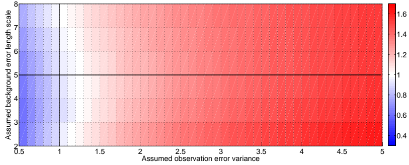
(a) Estimated observation error variance, \rho^e , as a function of assumed observation error variance and background correlation length scale. Red shows an overestimate, white an accurate estimate and blue an underestimate.
