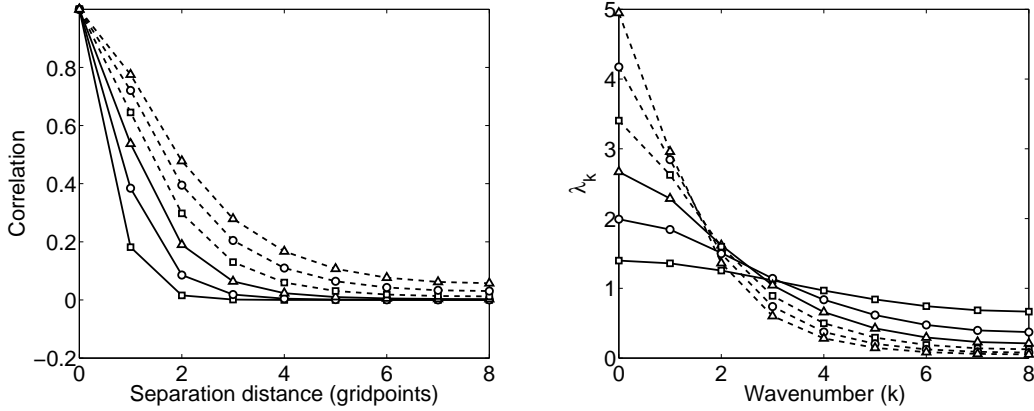
Figure 1: The SOAR function and its eigenspectrum. L = 2 (solid line squares), L = 3 (solid line circles), L = 4 (solid line triangles), L = 5 (dashed line squares), L = 6 (dashed line circles), L = 7 (dashed line triangles).
