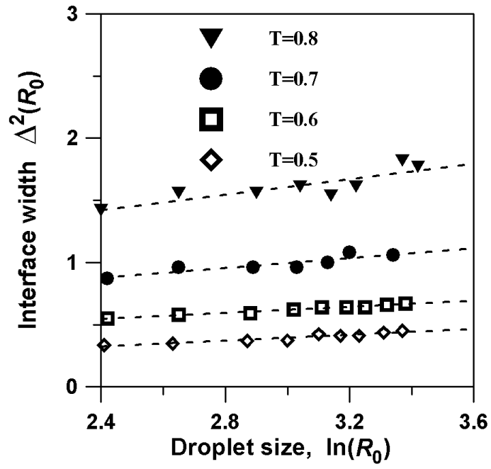
Figure 3: Interfacial width, \Delta^2 , as a function of the droplet size \ln(R_0) at different temperatures. The results of MD simulations are shown by symbols and the dashed line is the fit (3).
