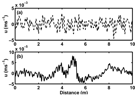
Figure 2: Plot (a) shows the error in the u field in the centre of time window for the assimilation with true linearization (dotted line) and approximate linearization (dashed line). Plot (b) shows the difference between the two solutions.
